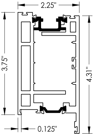
6 SASH
