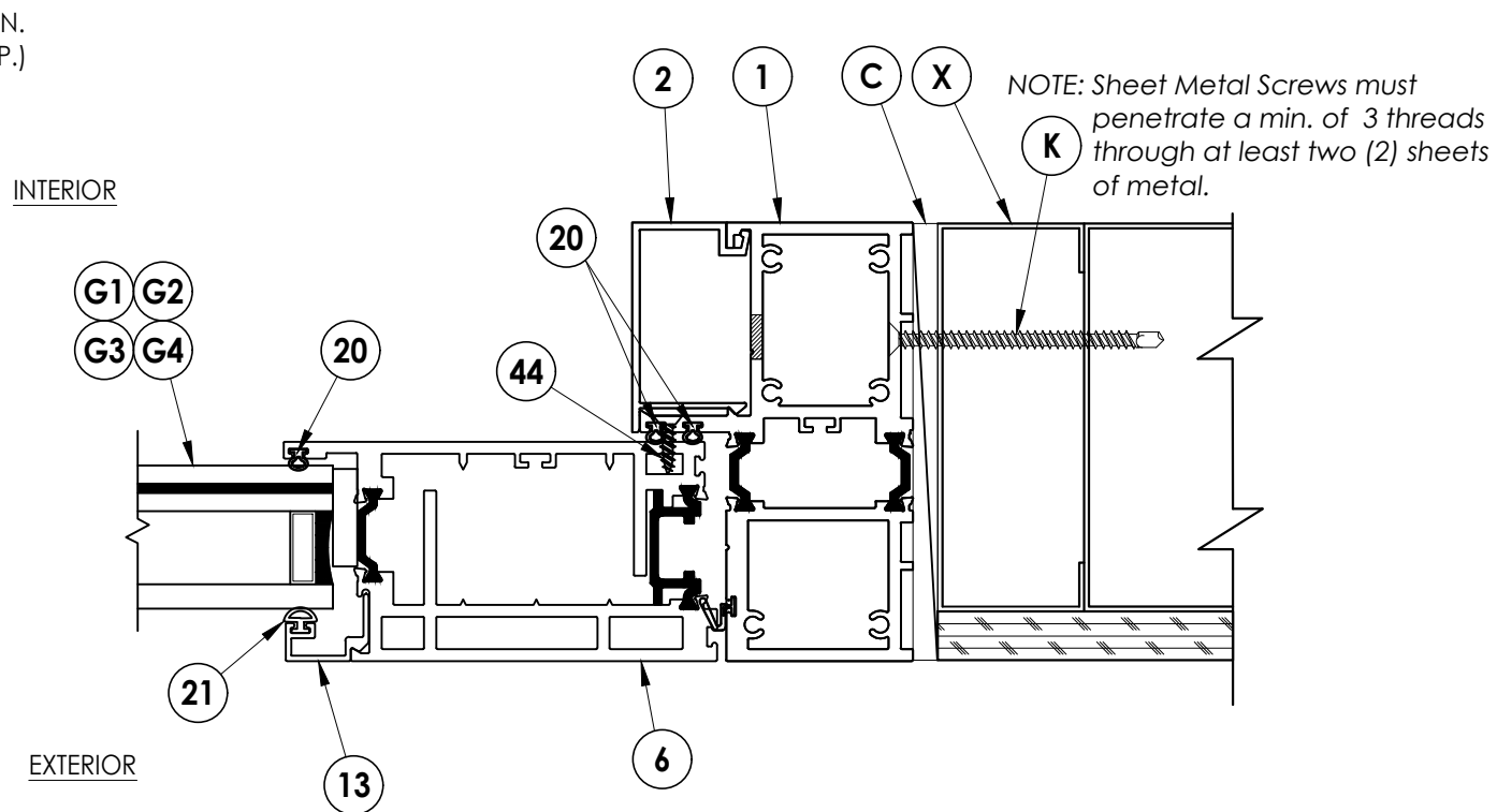
3 5 HORIZONTAL CROSS SECTION Metal Stud Construction Outswing Shown (Inswing Similar)
