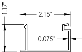
2 FRAME SNAP-IN
