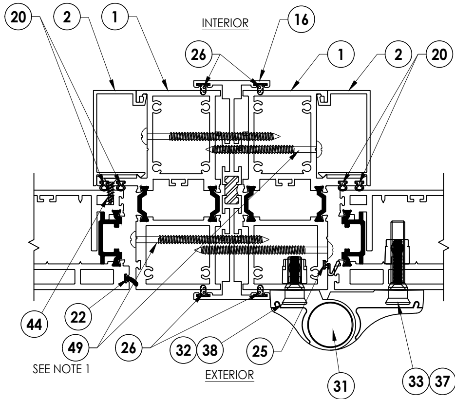
3 HORIZONTAL CROSS SECTION 6 Outswing Shown
