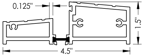
3 OUTSWING SILL
