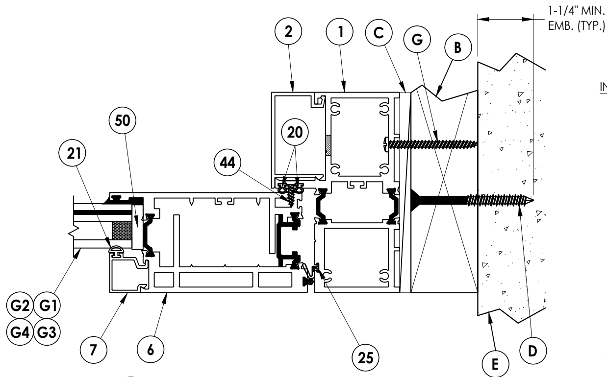
4 5 HORIZONTAL CROSS SECTION 2X Buck Construction Outswing Shown (Inswing Similar)
