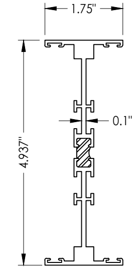
16 KONA I-MULLION
