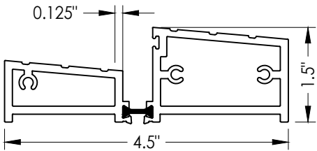
5 INSWING SILL
