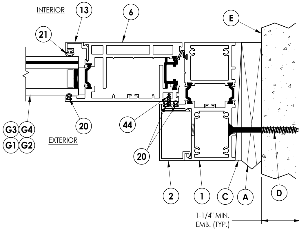
2 5 HORIZONTAL CROSS SECTION 1X Buck Construction Inswing Shown (Outswing Similar)
