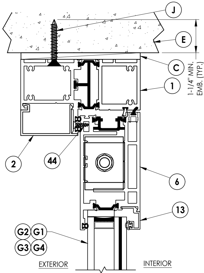
1 8 VERTICAL CROSS SECTION Inswing Shown
