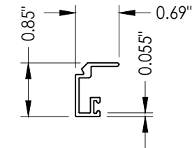
13 1.5" GLASS STOP
