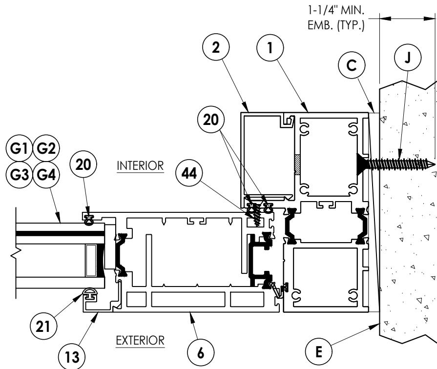
1 5 HORIZONTAL CROSS SECTION Direct to Masonry Outswing Shown (Inswing Similar)
