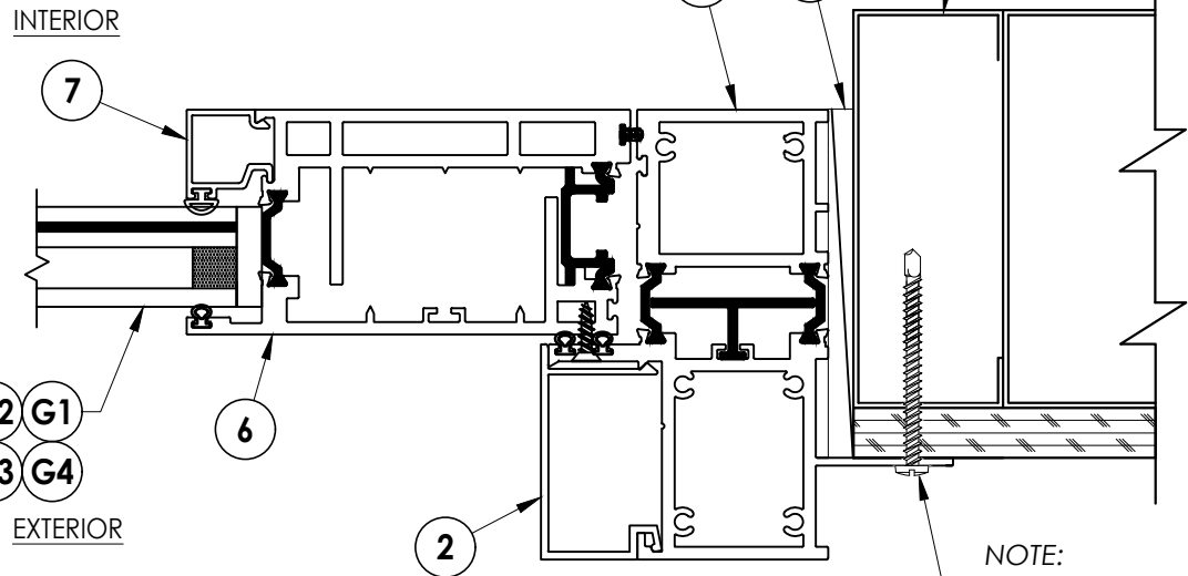
3 HORIZONTAL CROSS SECTION 9 Steel Stud Construction Inswing shown
