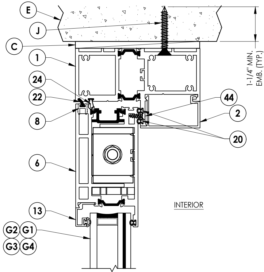
2 8 VERTICAL CROSS SECTION Outswing Shown
